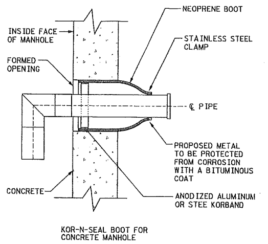
DETAIL NTS
