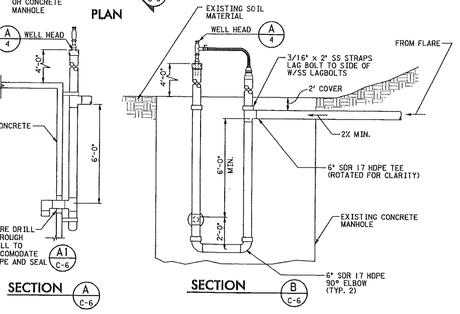
CONDENSATE LINE CONNECTION TO EXISTING MANHOLE DETAIL NTS
